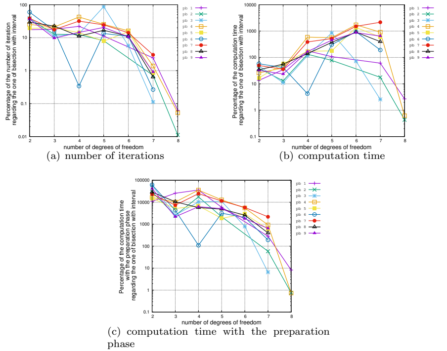
Figure 5: Comparison of the BSplines Contraction and the Interval Bisection methods to solve CSP.
