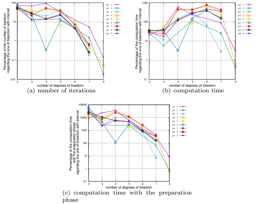
Figure 3: Comparison of the BSplines Bisection and the Interval Bisection methods to solve CSP.
